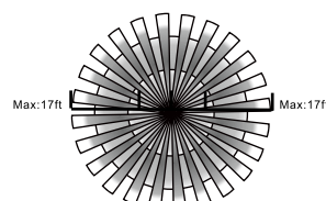
(Height of installation 8ft) Detection range
